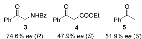
Figure 2. Asymmetric hydrogenation of other ketones: 3 , 4 with Pd(CF 3 CO 2 ) 2 /( R,R )-Me-DuPhos, and 5 with Pd(CF 3 CO 2 ) 2 /( S )-SYNPHOS.
